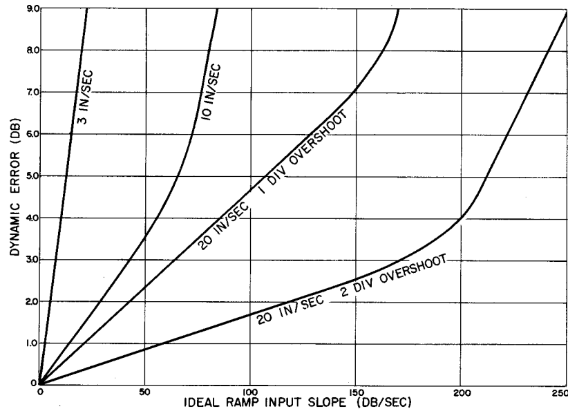
Figure 4.6. Dynamic error for various writing speeds (with 40-db potentiometer).
